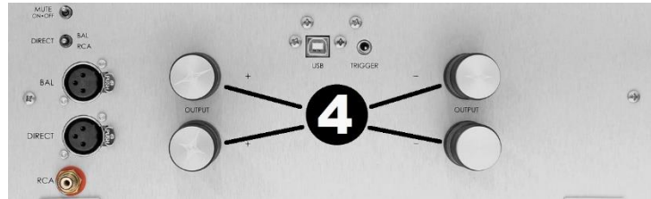
Inspiraton MONO 1.0 binding post layout
